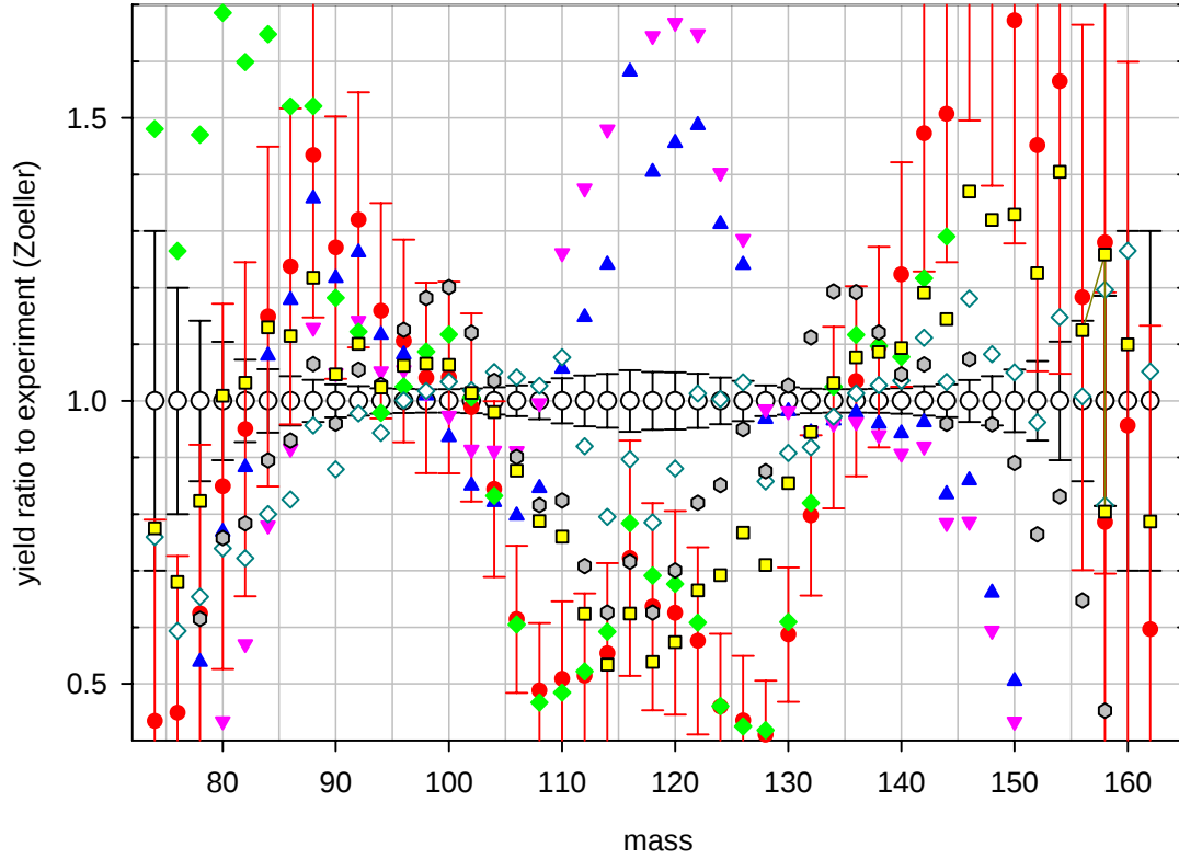
Benchmark A: ^{238}\text{U} around 13 MeV, post neutron emission yield ratio to experiment (Zoeller) lower graph: partial plot (high and low values omitted), for legend see upper graph.
